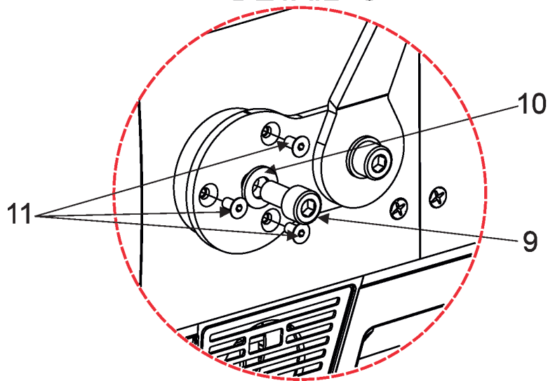
DETAIL C
